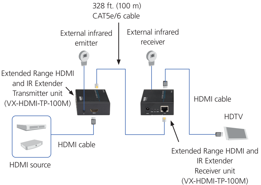
Figure 3-1. Connection diagram.
