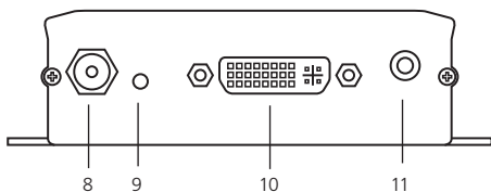
Figure 2-3. Receiver's front panel.
