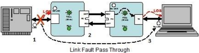
LFPT requires both TXLL and FXLL to be enabled.
