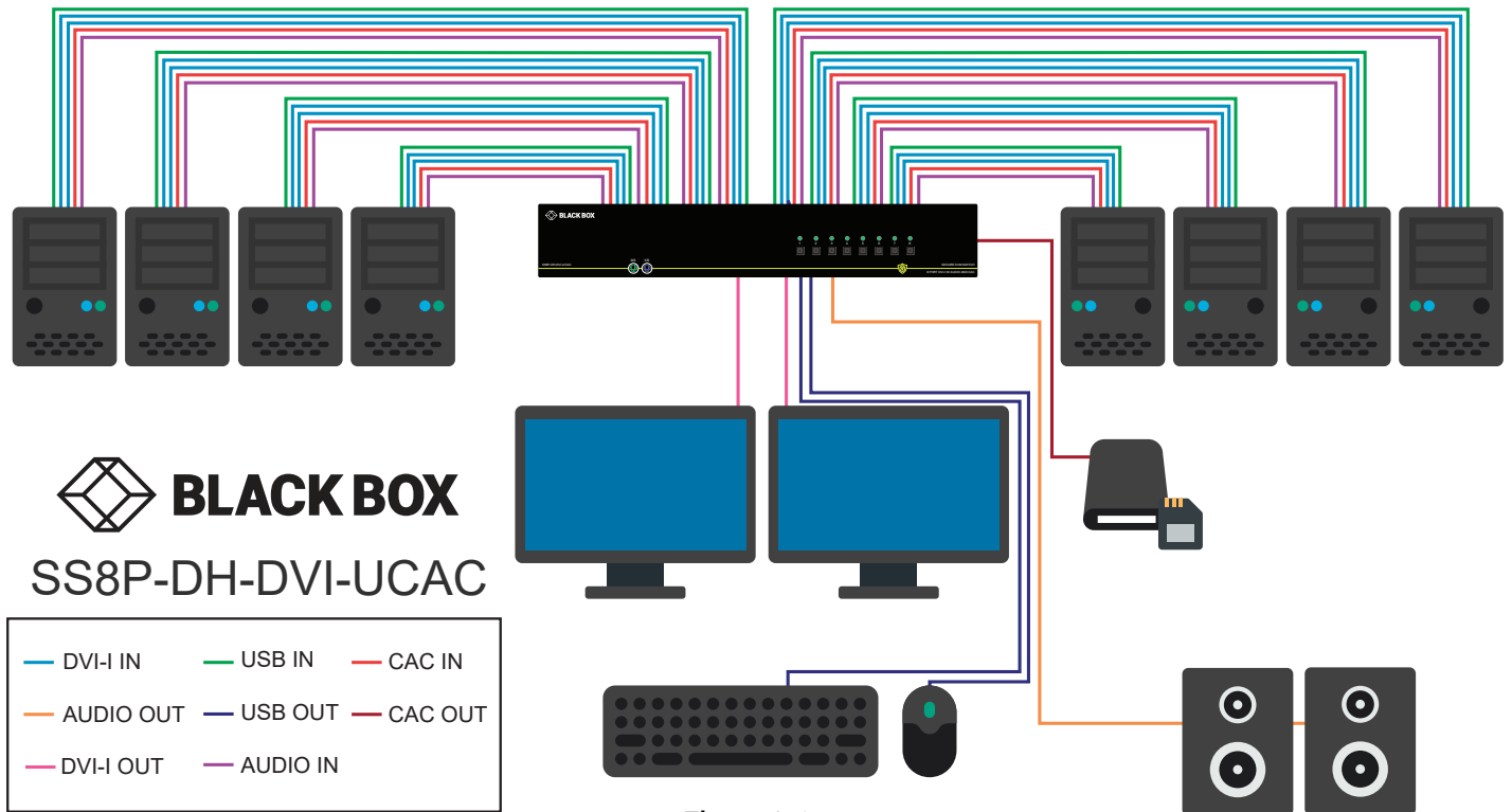
Figure 8-1 SS8P-DH-DVI-UCAC Shown
