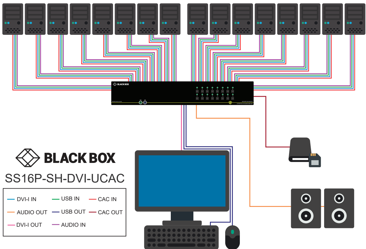
Figure 8-2 SS16P-SH-DVI-UCAC Shown
