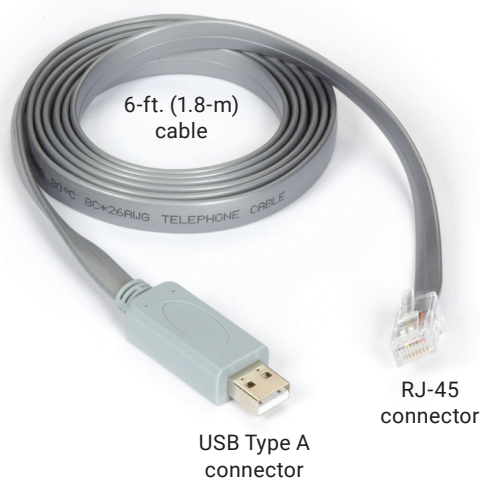
FIGURE 2-1. IC1101A
