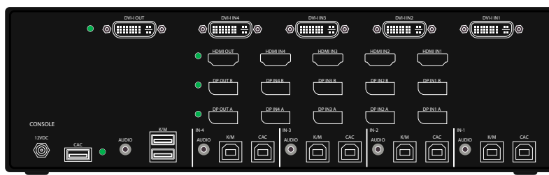
Figure 1-2: KVS4-1004VMX Rear panel
