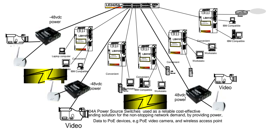
Example 4b. LP004A (Power Source Switch) for PoE device only
